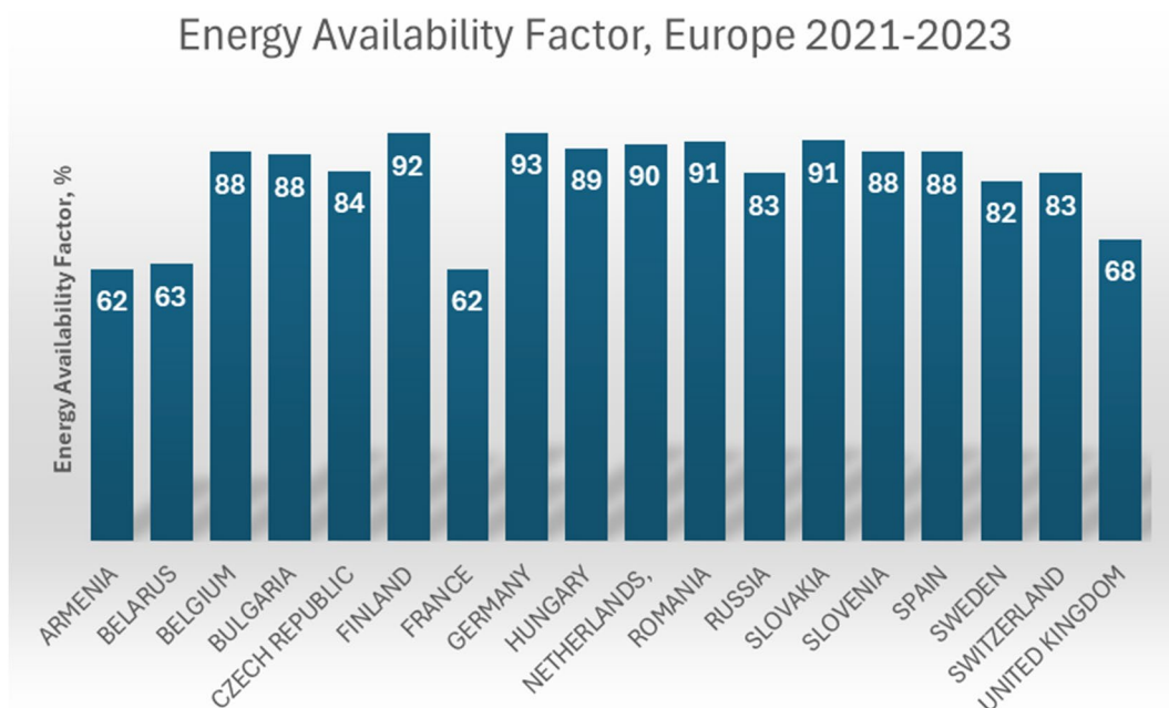
Figure 34 Nuclear reactor availability factor in Europe for 2021-2023 according to the IAEA 35
