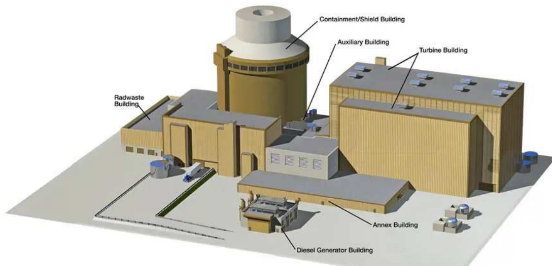
Figure 32 Layout of the main buildings of a nuclear power plant based on the AP-1000 reactor
