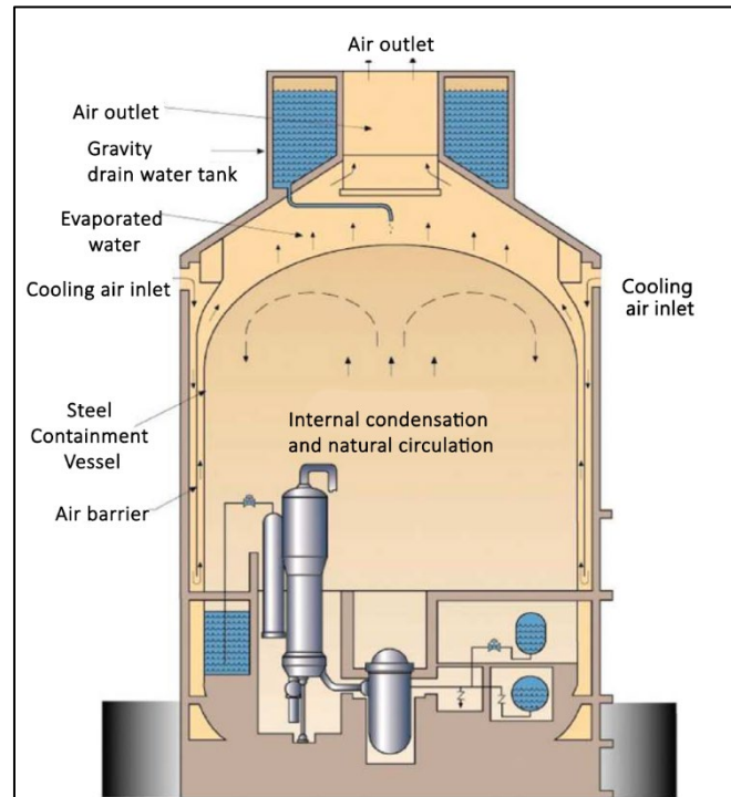
Figure 29 Reactor building
