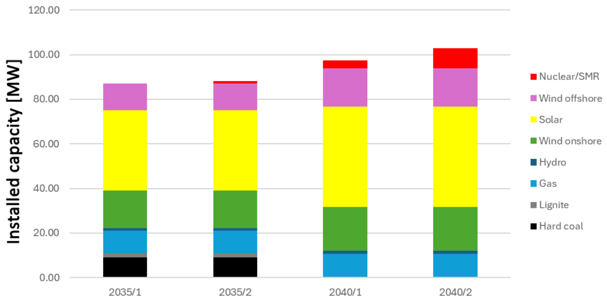
Figure 13 Forecast of generation source structures in 2035 and 2040
